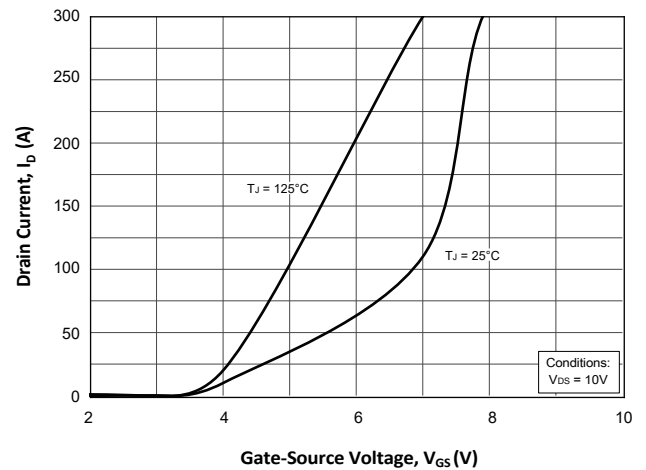
Fig.4 Transfer Characteristics
